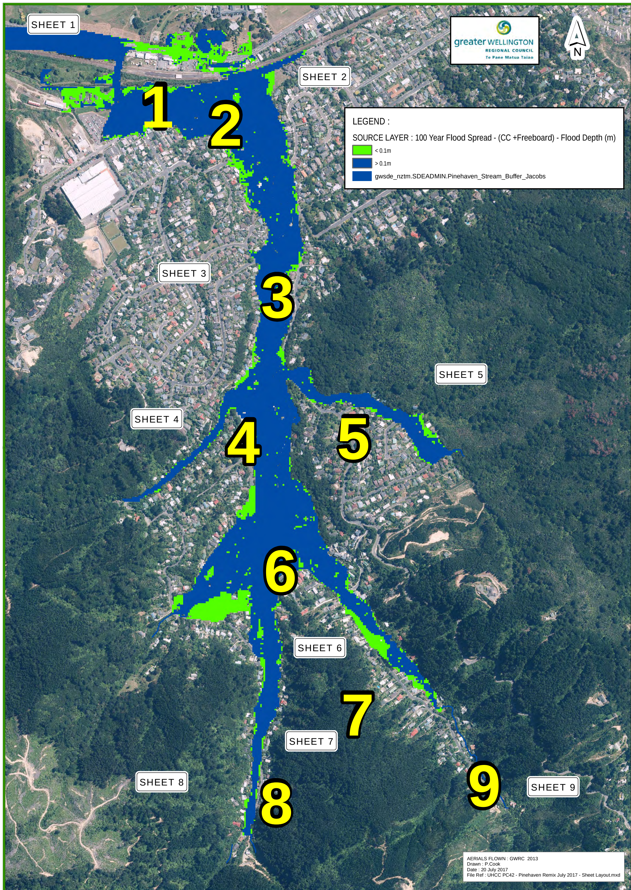
PINEHAVEN STREAM :UHCC PC42 REFINE (Flood Depth > 0.1m) SHEET LAYOUT
