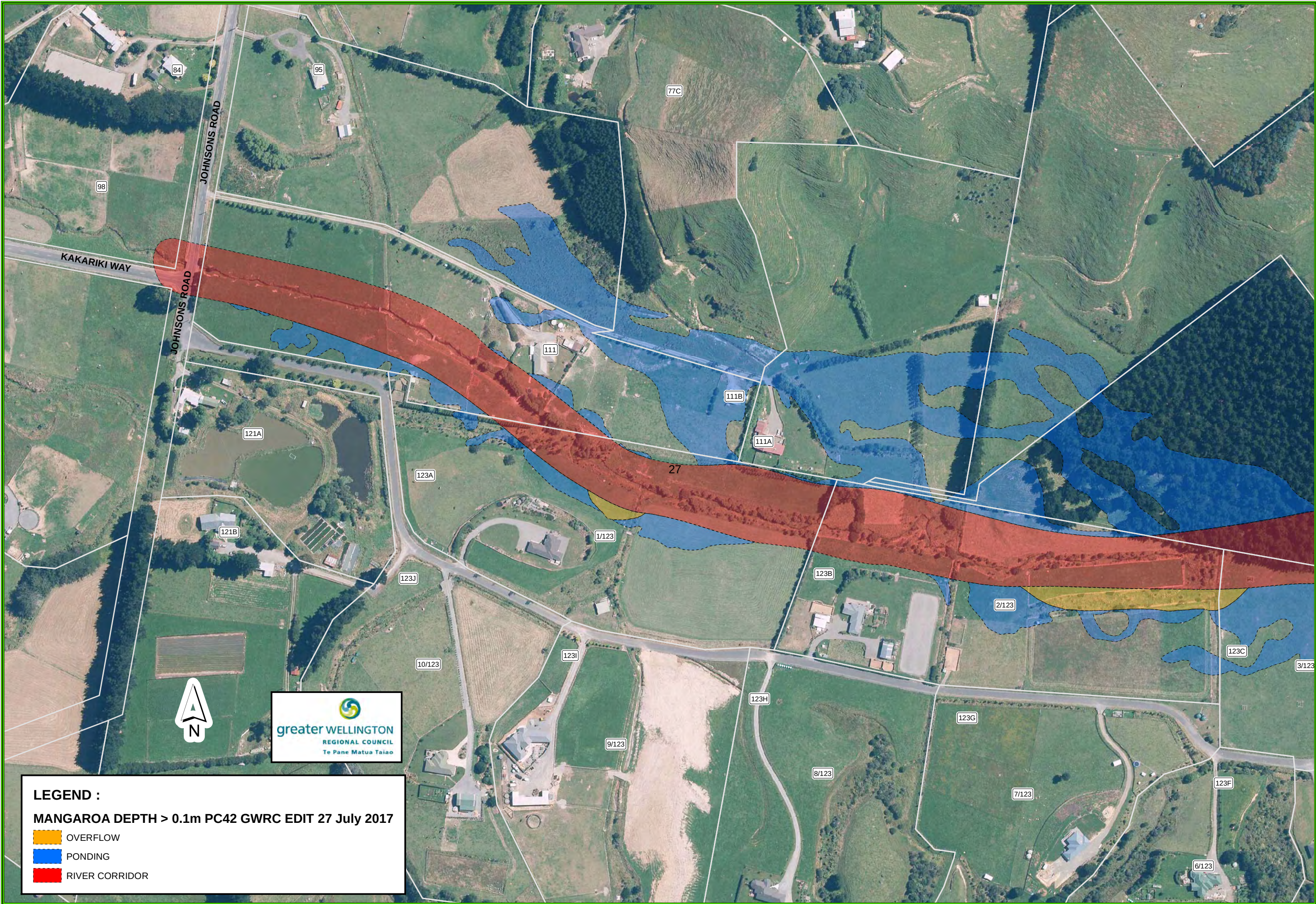
MANGAROA RIVER : UHCC PC42 REFINE (Flood Depth > 0.1m)
